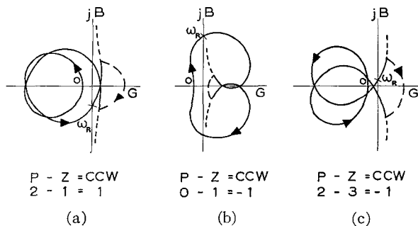
Fig. 5. Addition of Y_1(j\omega) to curves of Fig. 4.
