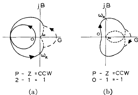
Fig. 4. Tunnel-diode admittance characteristics Y_D(j\omega) .
